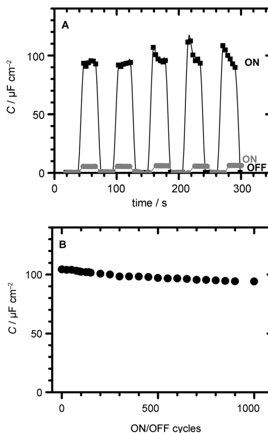
Figure 4. A) Comparative capacitance–time profiles at 50 Hz of the micropatterned Fc-modified surface (black) and the non-electroactive single-component butylamide-terminated monolayer-modified surface (gray) measured at 0.10 \pm 0.05 V during several dark (OFF)/illumination (ON) switching cycles. B) Stability of the photocapacitance measured at 50 Hz for an applied potential of 0.06 V vs. SCE as a function of the number of ON/OFF cycles. Illumination with white light was generated using a 50 W tungsten halogen lamp.
